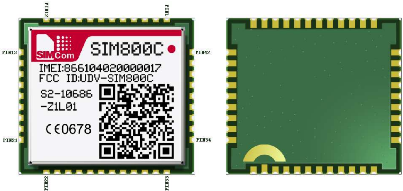
Figure 40: Top and bottom view of SIM800C
