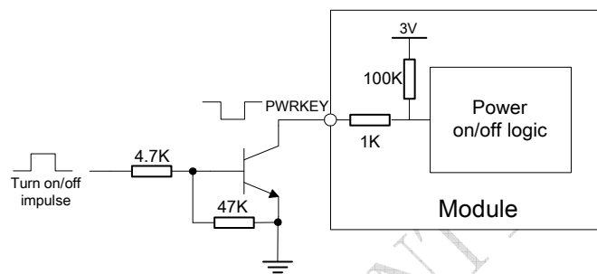
Figure 10: Powered on/down module using transistor
